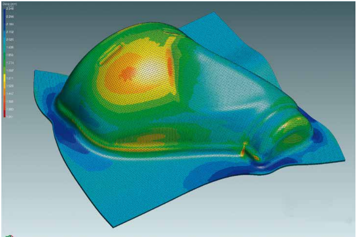
No problem even with thick-walled sheet metal: Stampack calculates multi-stage forming processes completely in volume. Here the simulation of the component of an exhaust system finished article see cover picture. (© Fütterer)
